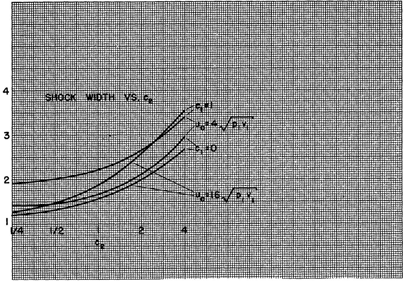
Fig. 7 Shock width vs. c_2 .
