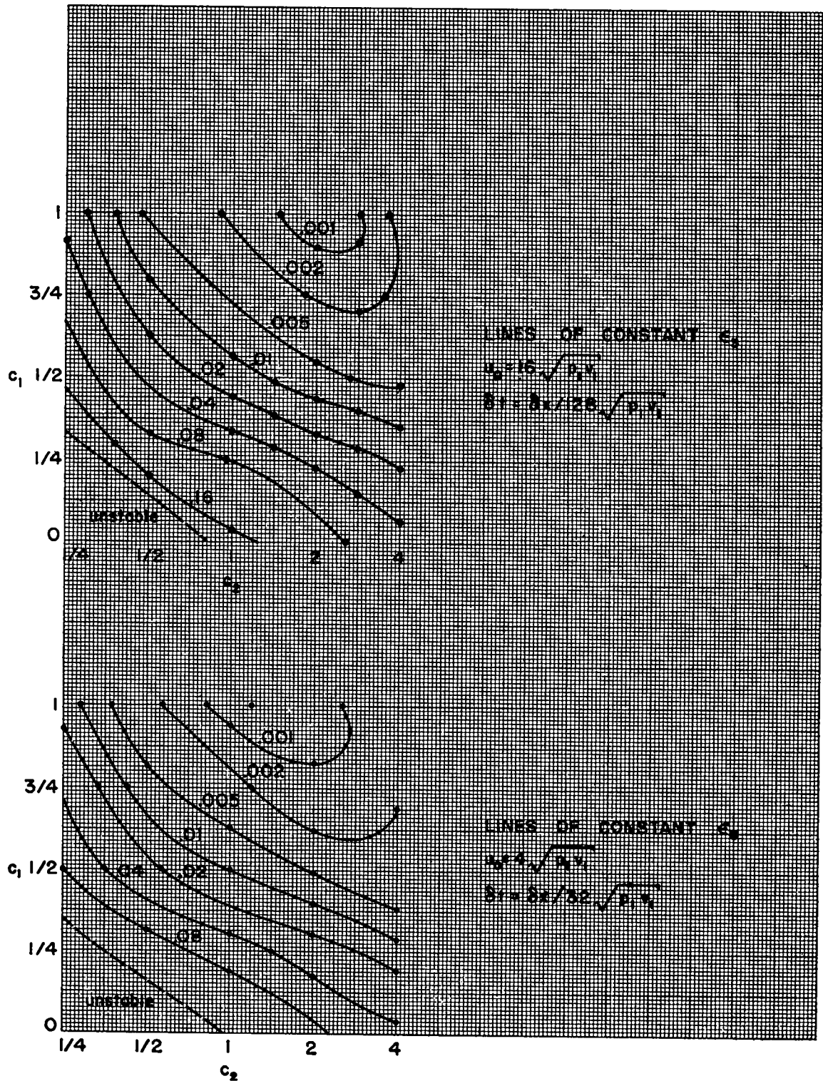
Fig. 6 Lines of constant \epsilon_3 in the c_1, c_2 plane.
