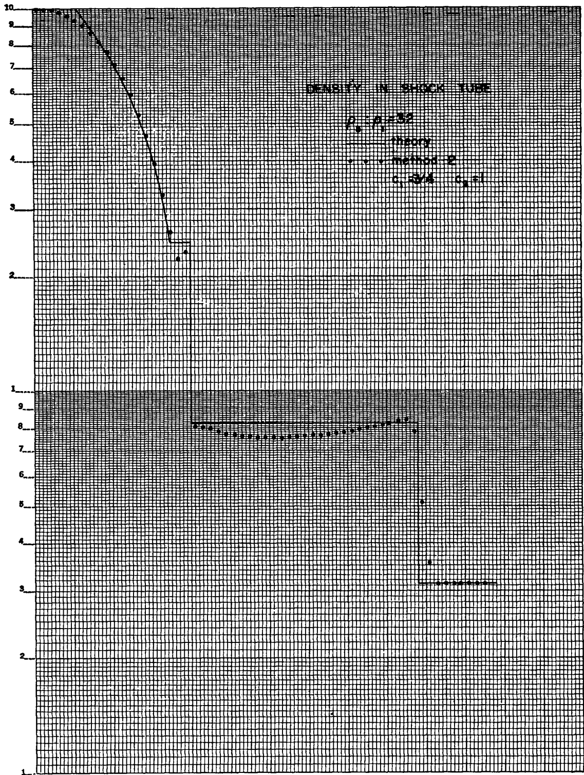
Fig. 15 Density in shock tube.
