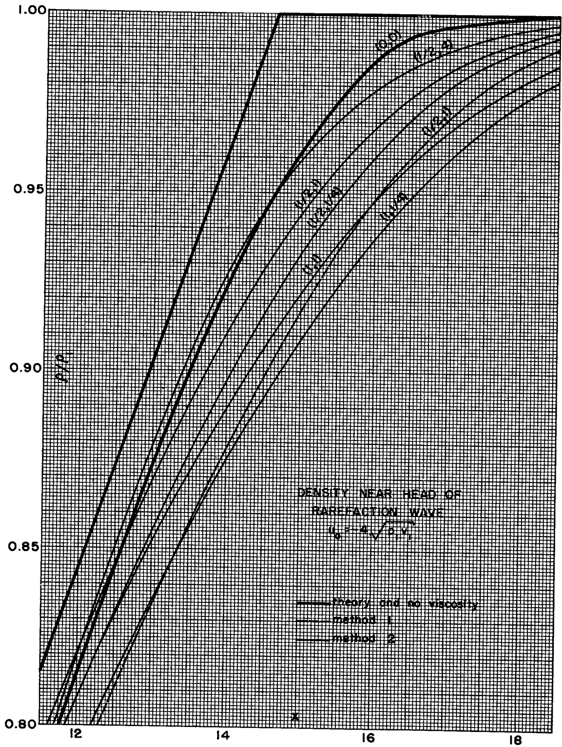
Fig. 13 Density near head of rarefaction wave.
