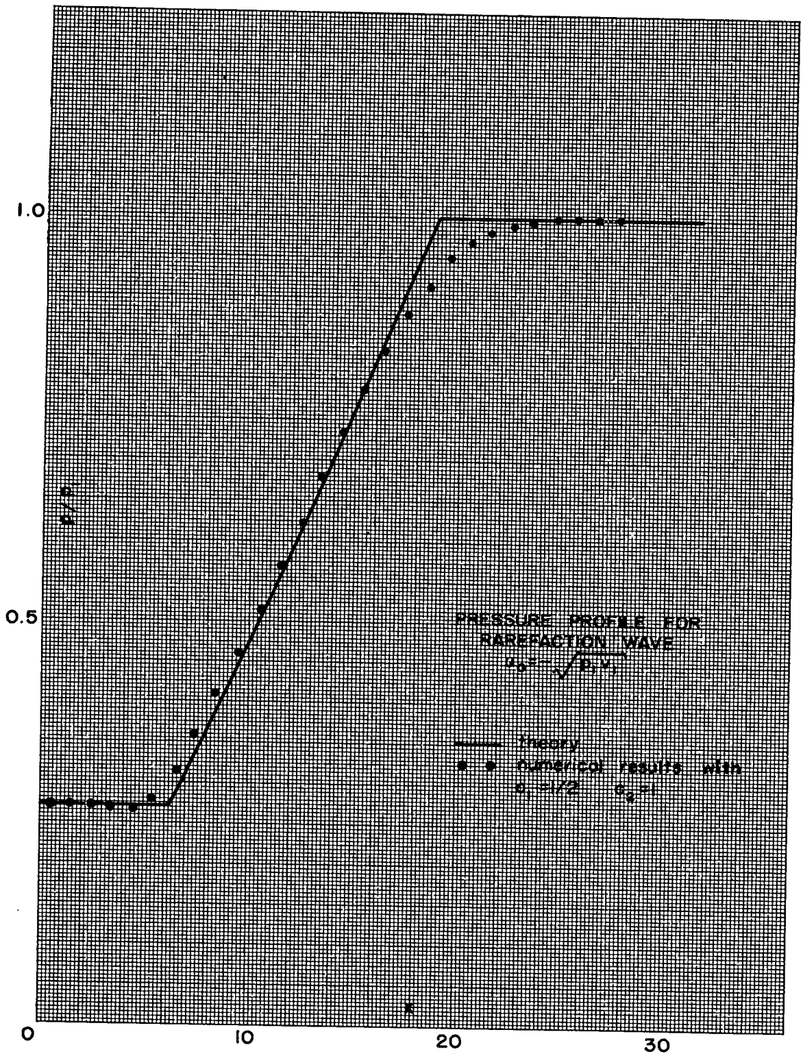
Fig. 11 Pressure profile for rarefaction wave.
