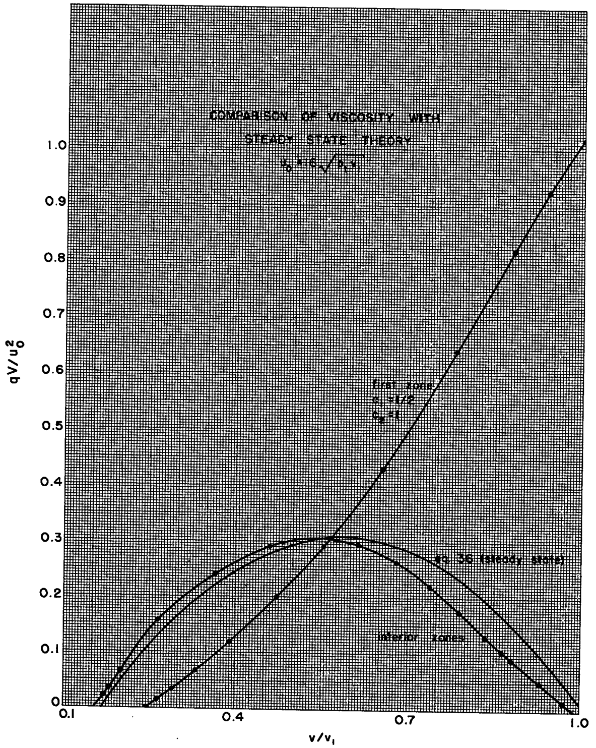
Fig. 8 Comparison of viscosity with steady state theory.
