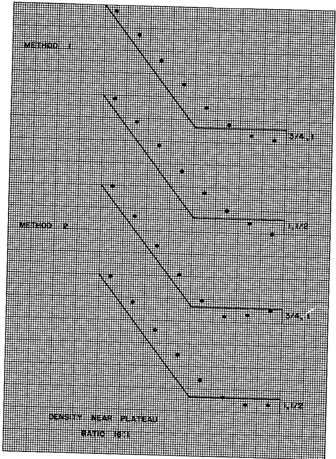
Fig. 16 Density near plateau.
