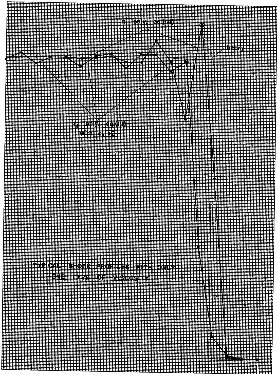
Fig. 4 Typical shock profiles with only one type of viscosity.
