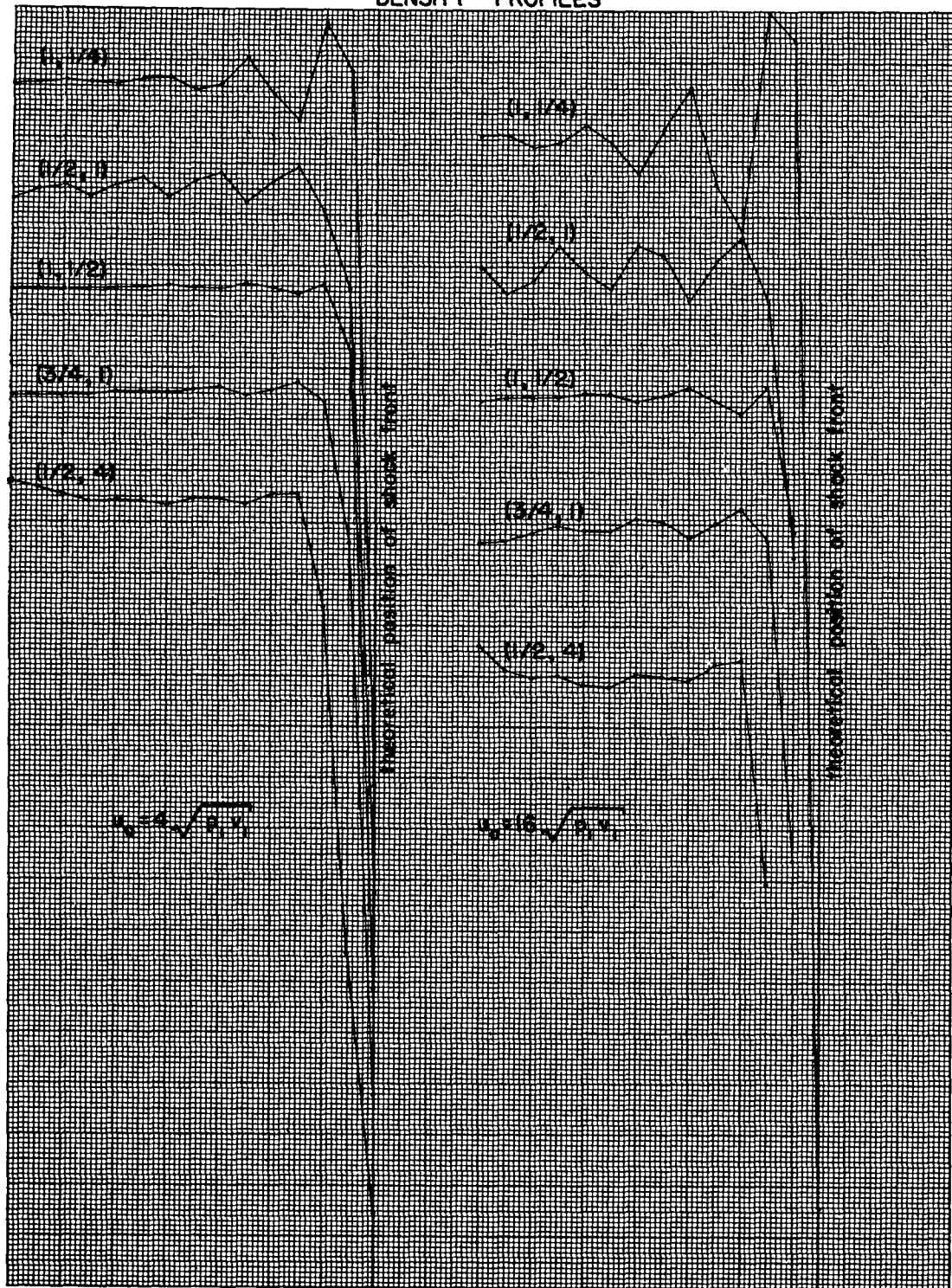
Fig. 10 Density profiles for selected combinations of c_1 and c_2 .
