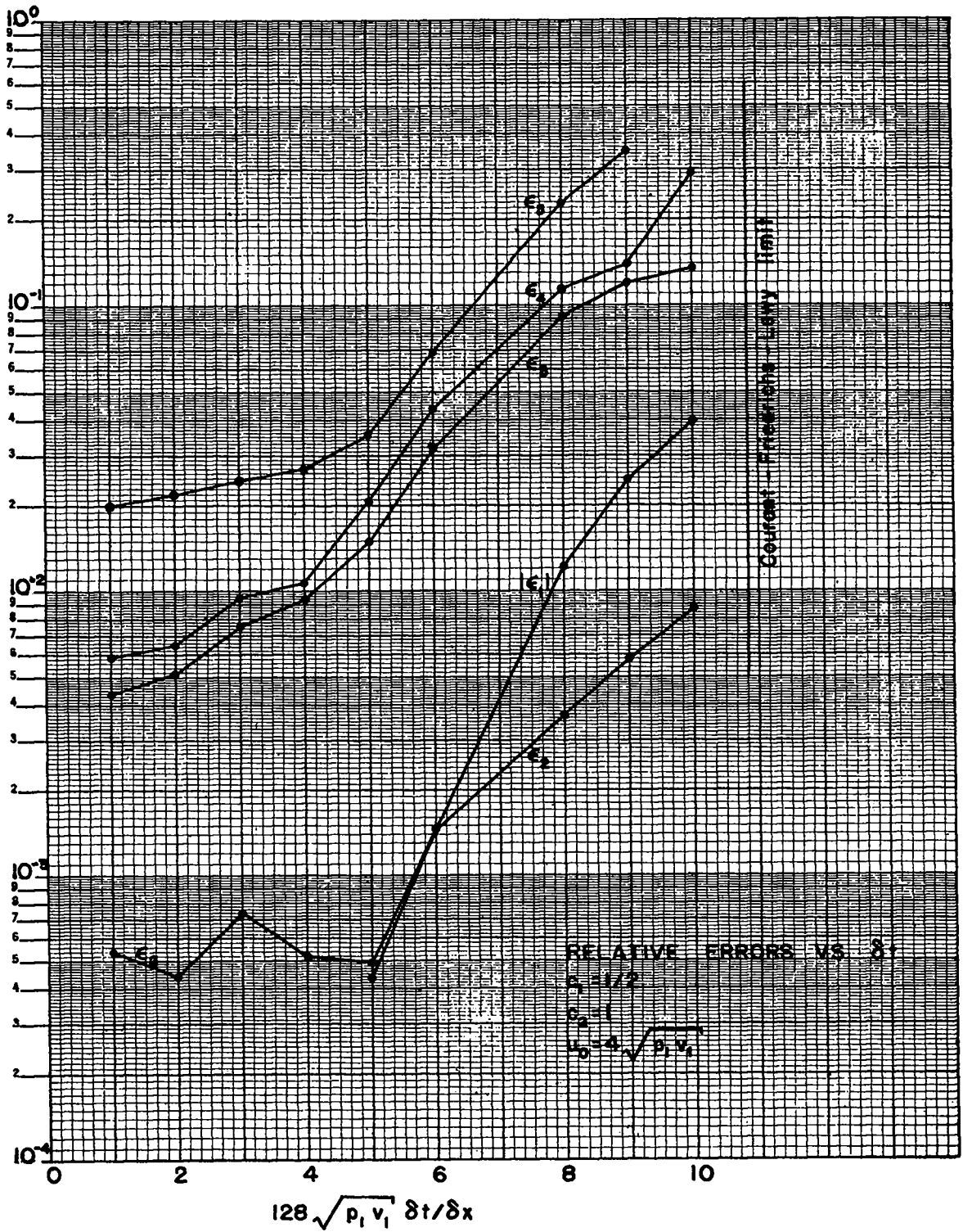
Fig. 5 Relative errors vs. \delta t .
